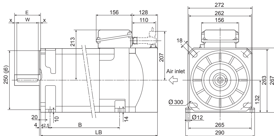
Motor AMS 132
