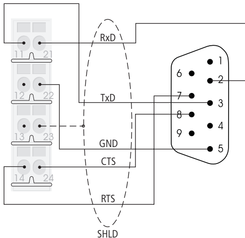
Figure 4: Wiring diagram for XN-S4x-SBBS and submini D plug (top view)
