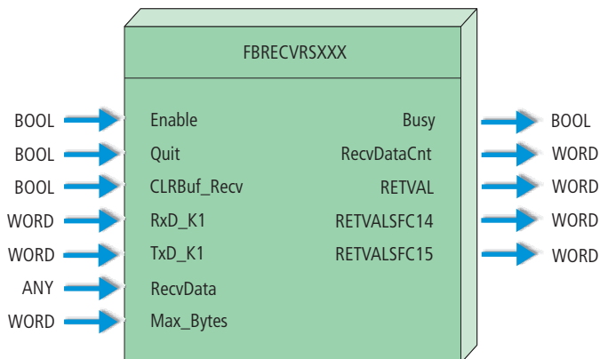
Figure 6: Receive function block for the SIMATIC S7 software
