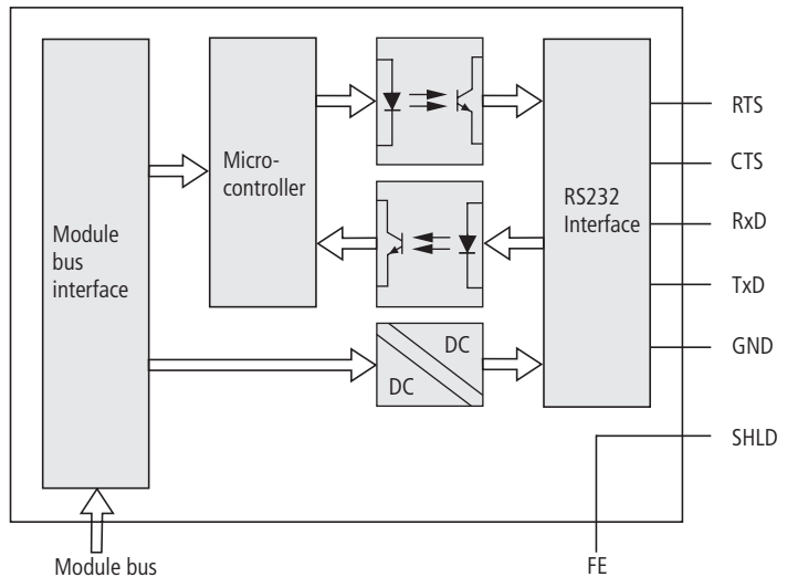
Figure 2: Block diagram of the XN-1RS232 module
