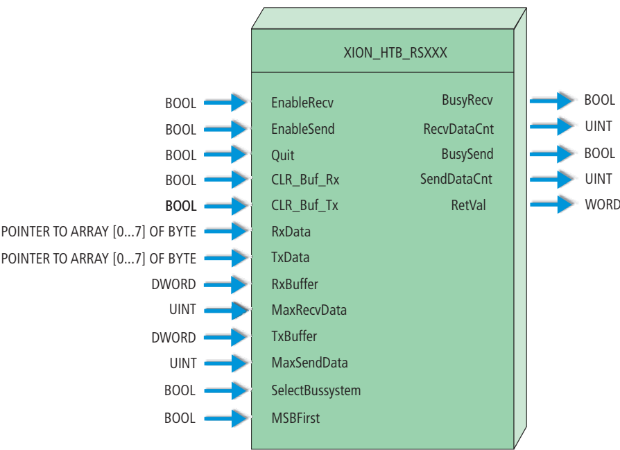
Figure 9: Transmit/receive function block for the CoDeSys software MXpro
