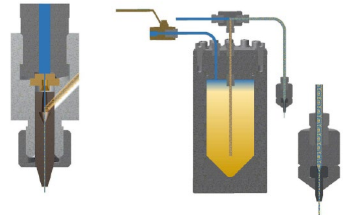
In injector technology, water is fed under pressure through a nozzle into a mixing chamber where it generates a vacuum that sucks in and accelerates abrasive. In suspension technology, water and abrasive are mixed and then pressurized together.
