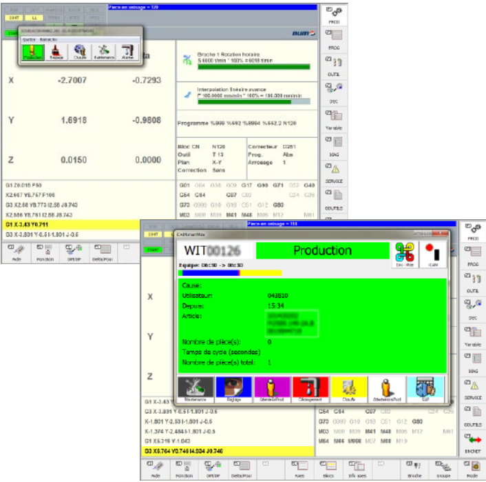
Integration of iCAMNet in NUM HMI in 2 variants.
