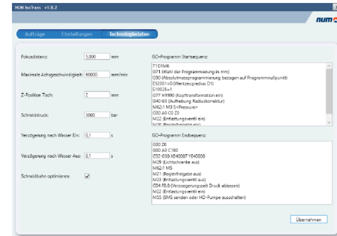
Screenshot of the NUM IsoTrans technology data.
