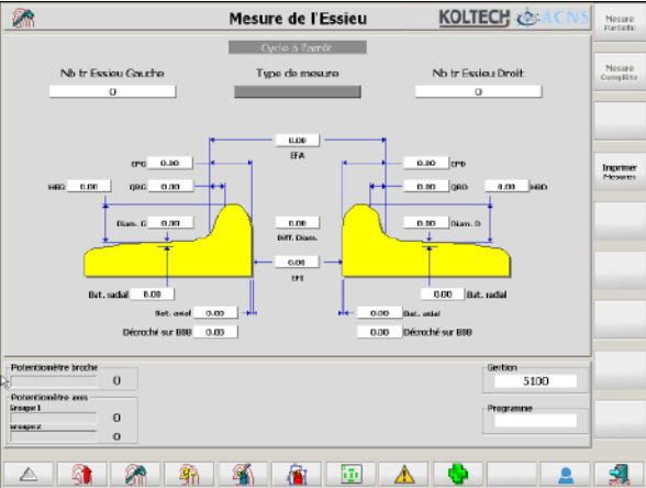
An example of a page from the Man-Machine interface Axle measurement.
