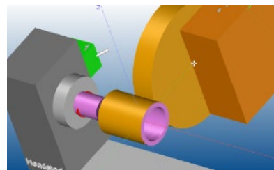
Wheel change and OD traverse cycle G206 at surface of the tube part.
