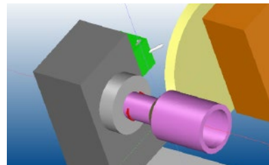
Processing start of OD conical traverse cycle G210 at inclined shaft part.
