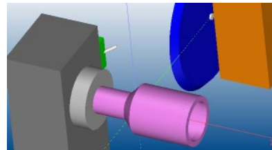
Blank formed as shaft and tube.
