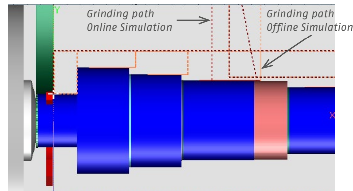
Processing start of OD conical traverse cycle G210 at inclined shaft part.
