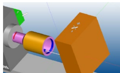
Wheel change and ID traverse cycle G207 at inside of the tube part.
