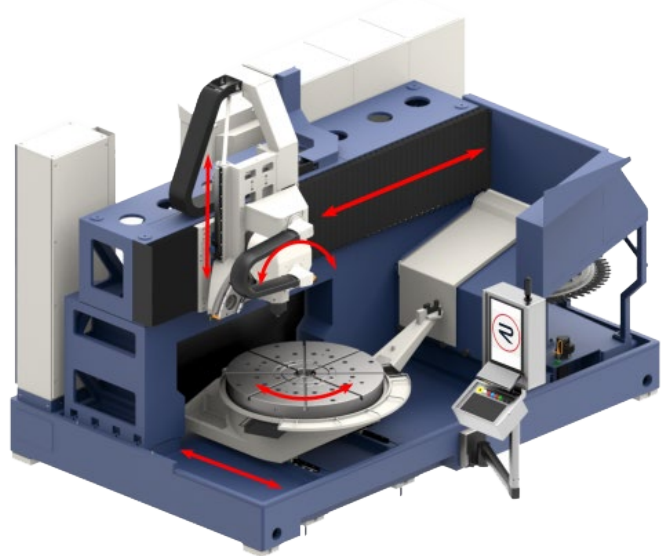
Machine axis overview.
